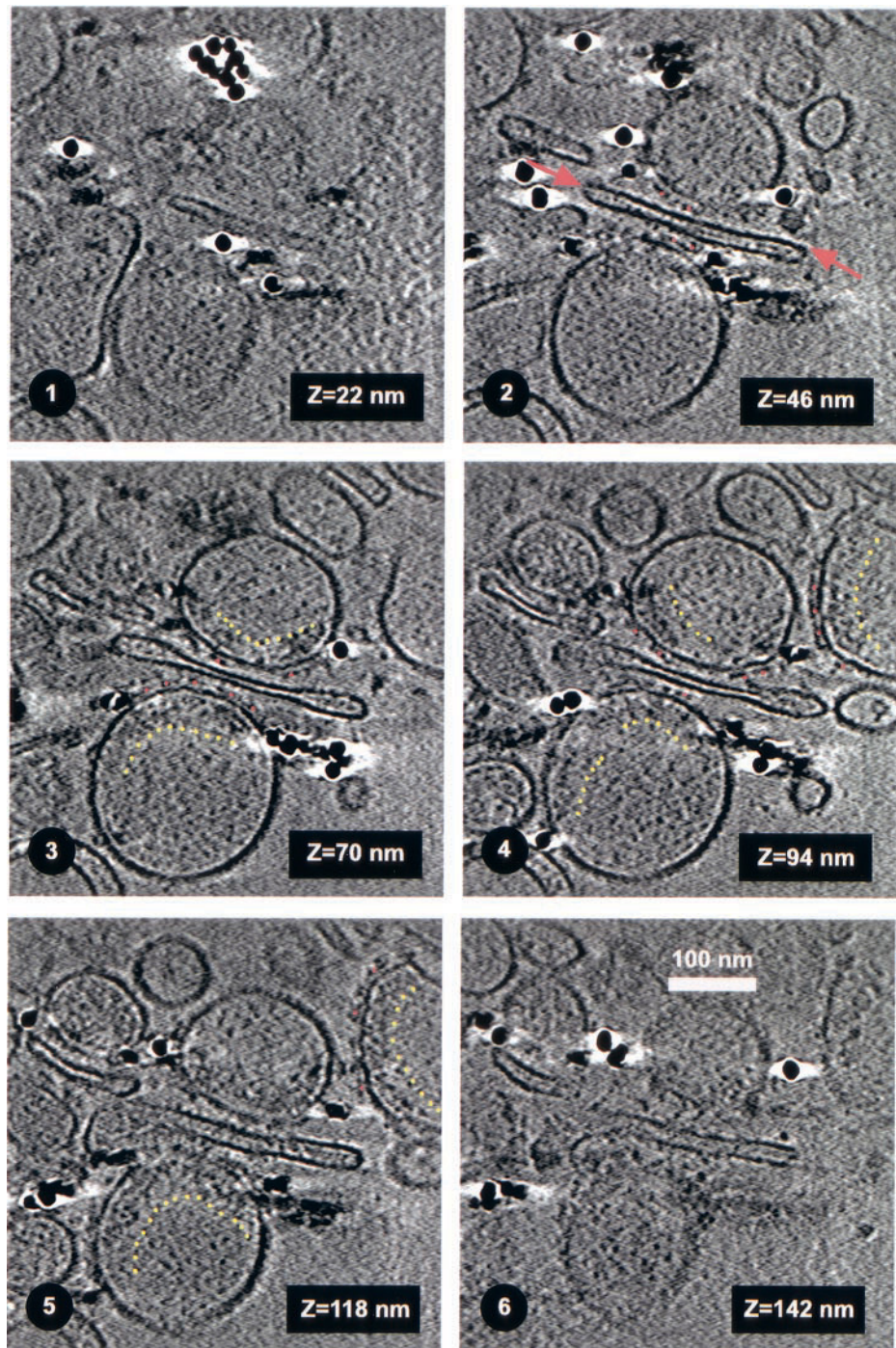
FIGURE 3 Selected XY-slices from tomographic reconstruction of triad 3. The Z-coordinate of each slice is indicated in lower right corner. Orange dots denote locations of RyRs (feet); yellow dotted lines are drawn to indicate regions of organized calsequestrin located between the dotted line and the SR membrane. The TC vesicle at upper right in panels 4 and 5, which is not part of the triad, contains particularly well-resolved RyRs and underlying organized calsequestrin. Notice that the colloidal gold clusters are present in all slices, indicating that the clusters are distributed uniformly throughout the layer of vitreous buffer in which the triads are embedded.
